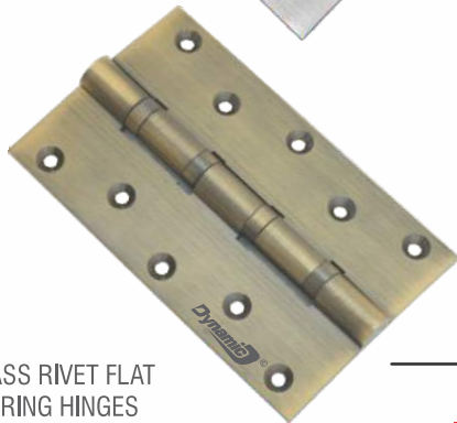
Pin Locking System Steel Pin locked between Brass Rivets at top and bottom for extra safety for doors & windows
